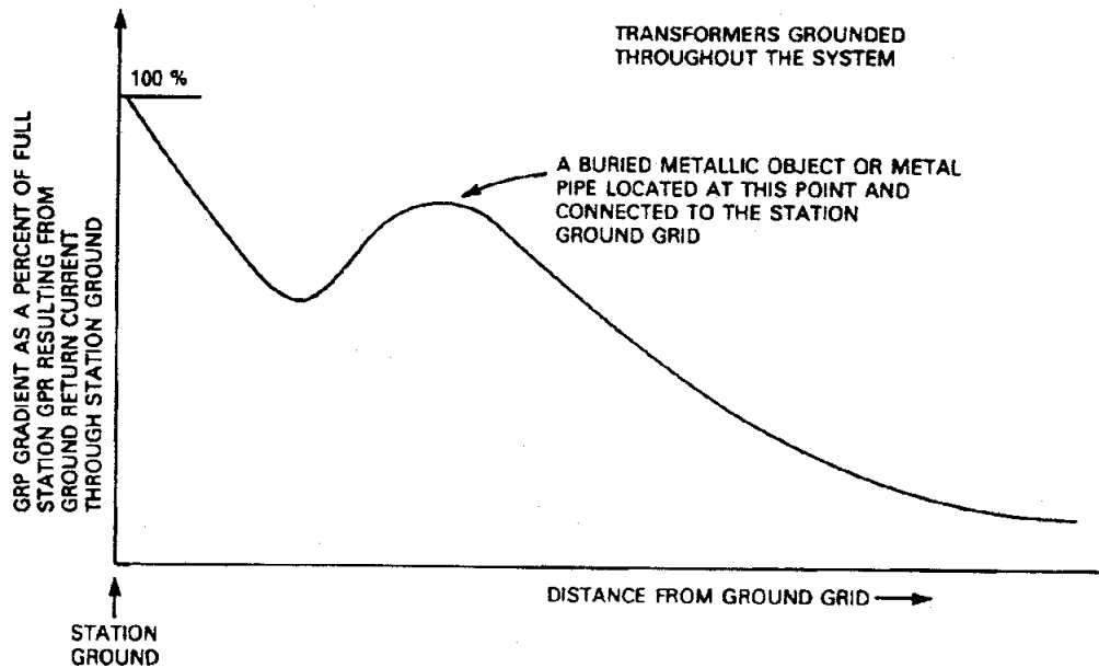
Figure 43b—Ground potential gradient
